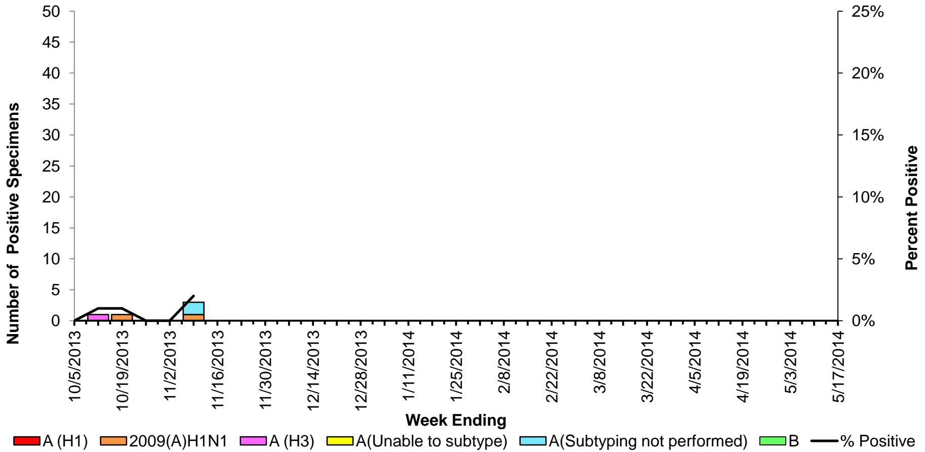
Influenza Isolates from Illinois Reported by WHO/NREVSS Collaborating Laboratories 2013-2014 Influenza Season
